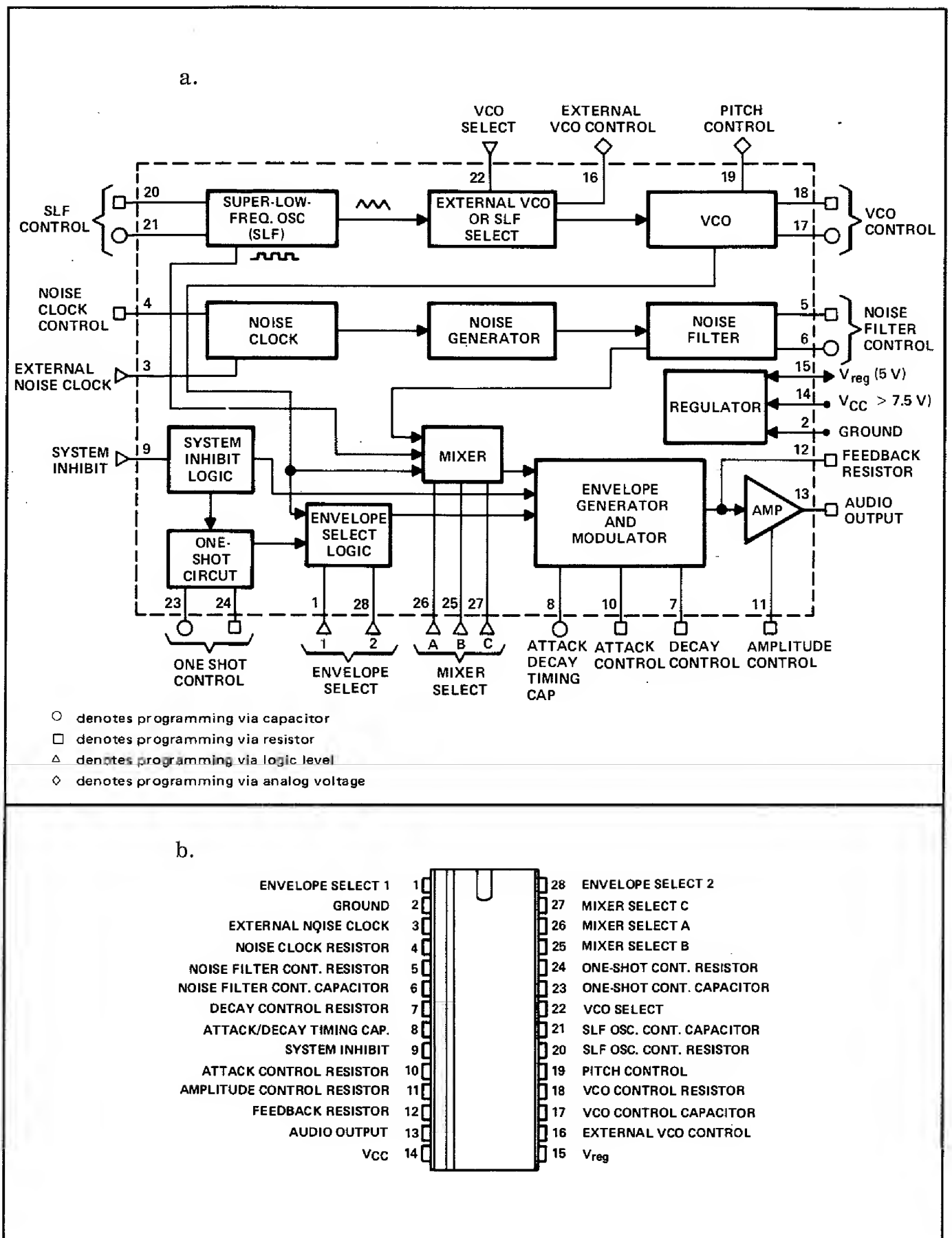
Fig 5.16 Ljudgenerator 76477N a. Blockschema b. Kapsel
