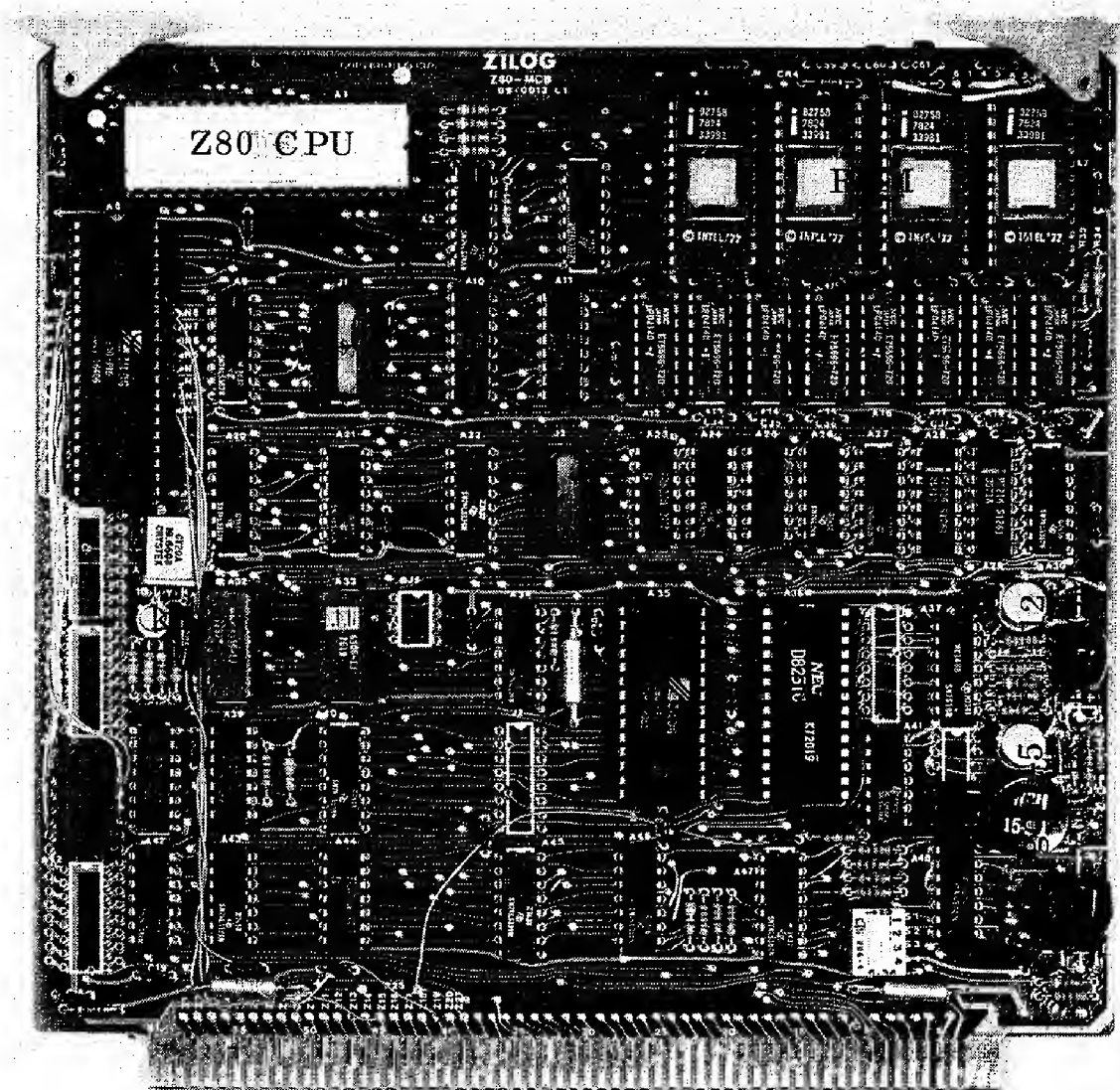
Fig 4.5 Z80-MCB
