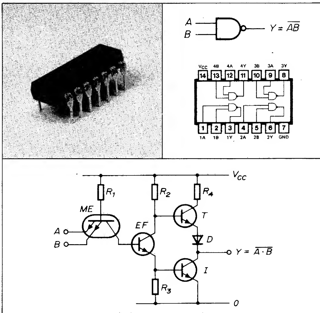
Fig 2.6 NAND-grinden 7400
