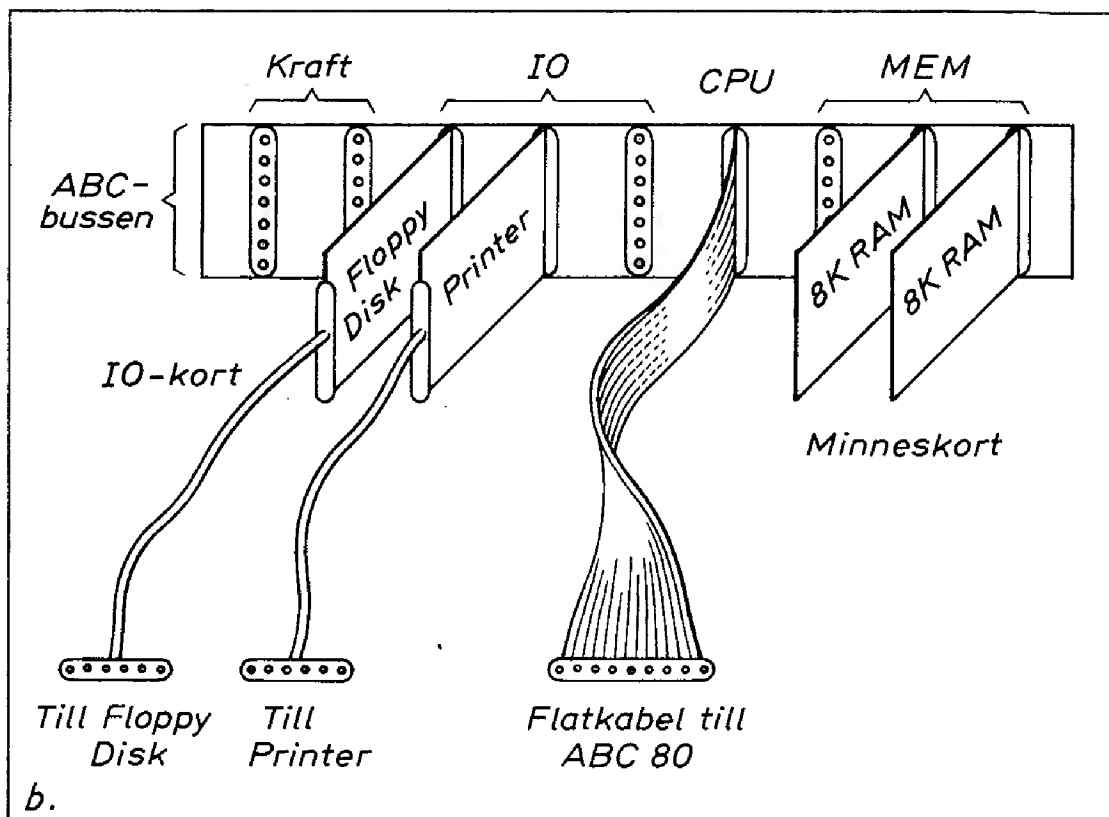
Fig 6.32 ABC-bussen
